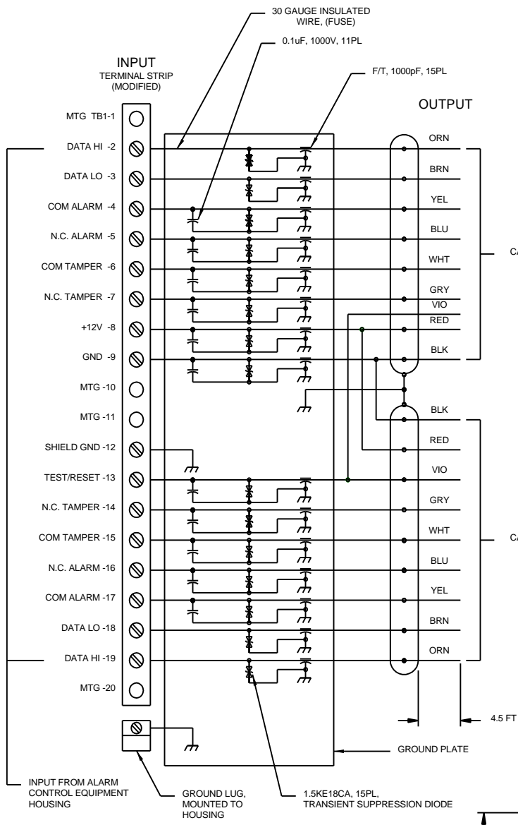
SCHEMATIC DIAGRAM
