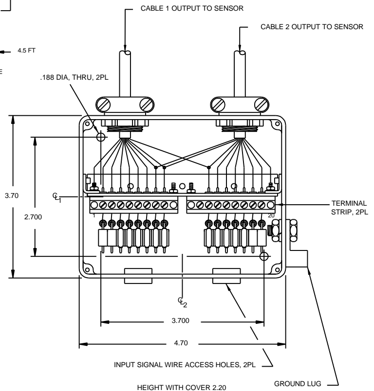
MECHANICAL CONFIGURATION
