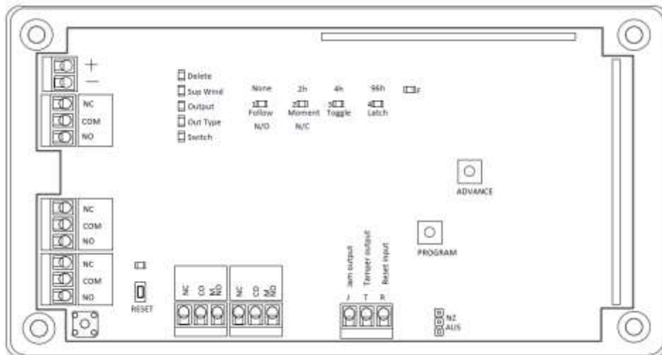
Wireless Receiver (62B47313-A01), internal view
