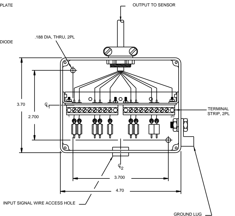
MECHANICAL CONFIGURATION
