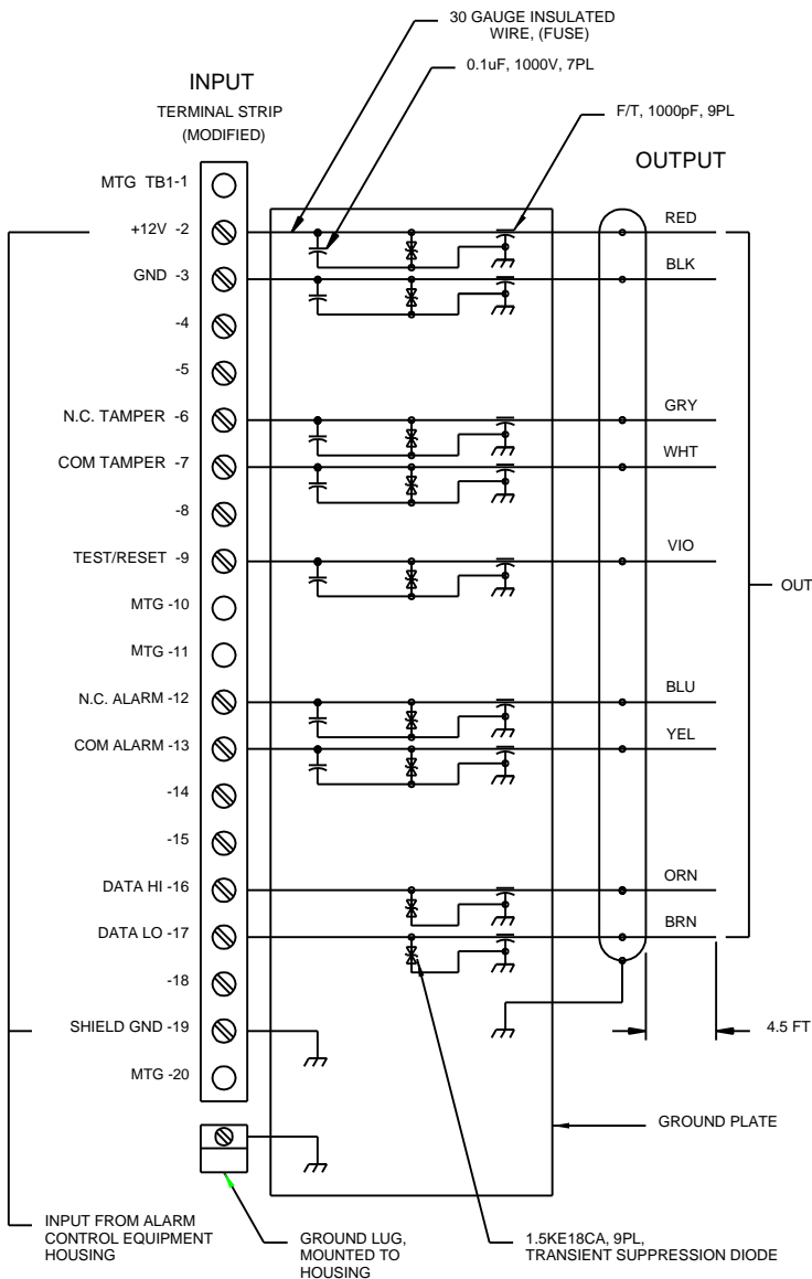
SCHEMATIC DIAGRAM
